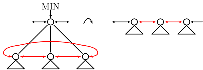
Abbildung 2.55: Skizze: Operation delete_min
